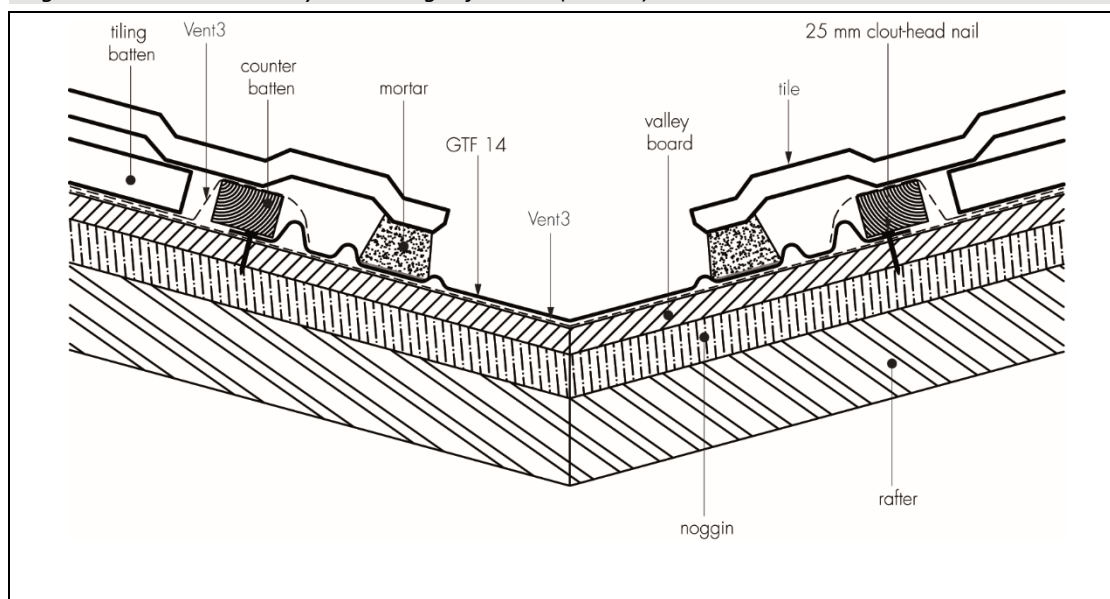
Figure 1 Cromar Pro Valley GRP Troughs for Tiles (GTF 14) – Flat Fix
