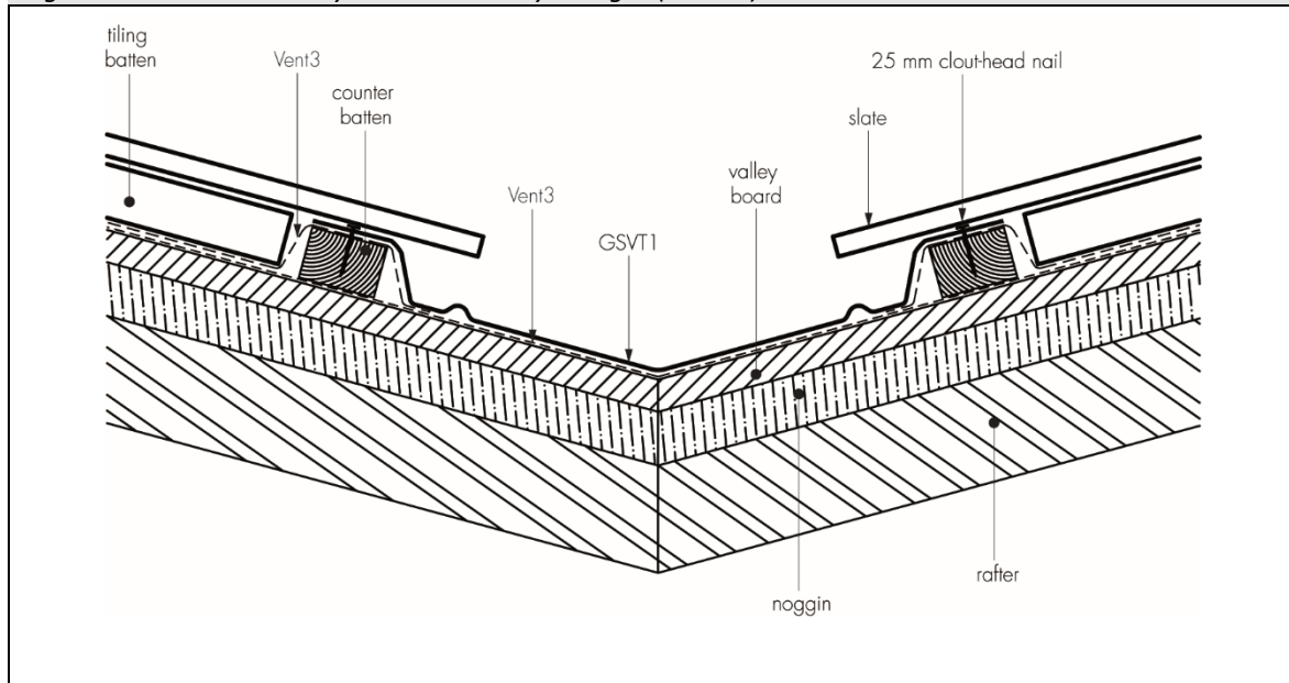
Figure 1 Cromar Pro Valley GRP Slate Valley Troughs (GSVT 1)
