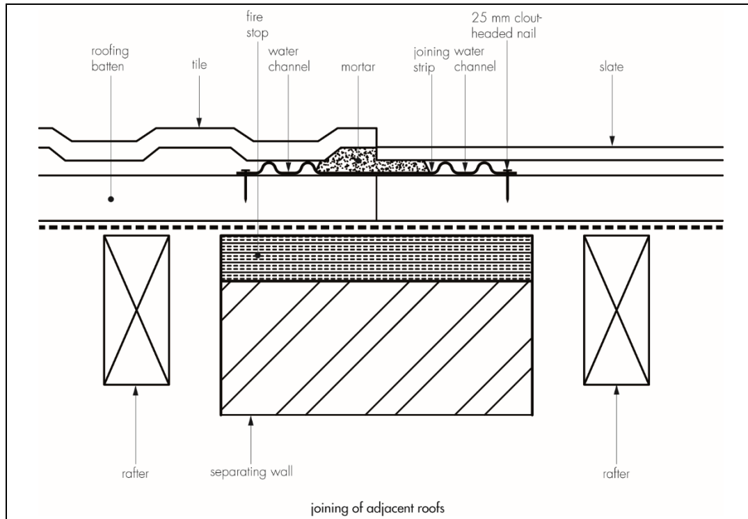
Figure 1 Cromar Pro Valley GRP Secret Joining Strip (GJS 1)
