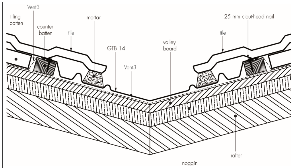
Figure 2 Cromar Pro Valley GRP Valley Troughs for Tiles (GTB 14) - Batten Fix
