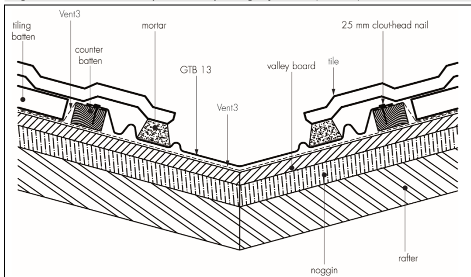
Figure 1 Cromar Pro Valley GRP Valley Troughs for Tiles (GTB 13) - Batten Fix
